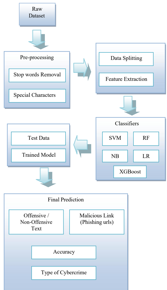
Fig3. Proposed Model
