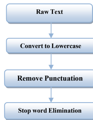
Fig 2 Data Preprocessing
