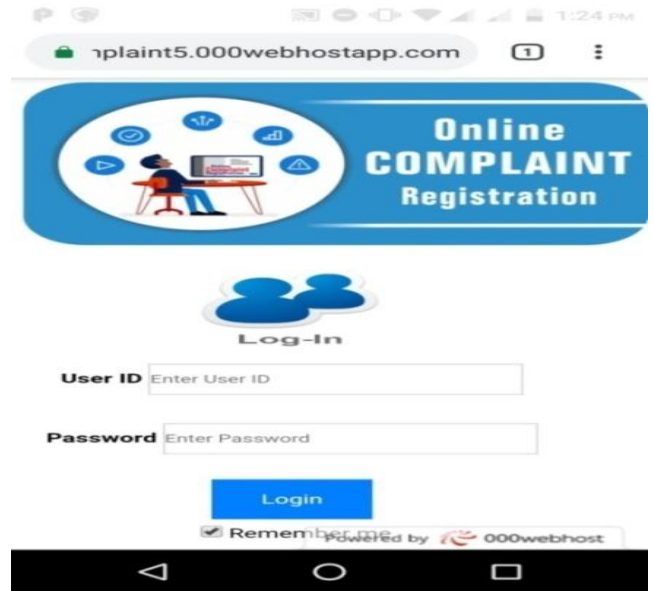
Fig.4. Login Form
