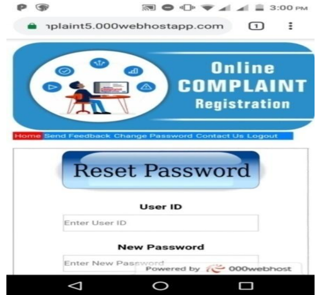
Fig.8.Change Password
