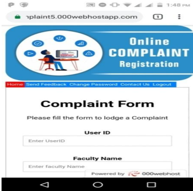
Fig.6. Complaint Form
