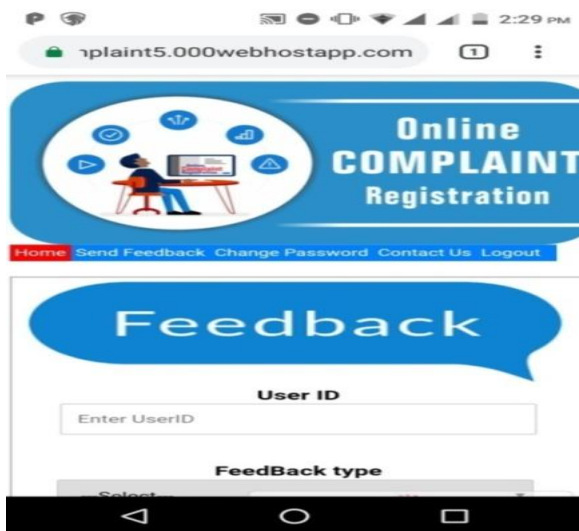
Fig.7. Feedback Form
