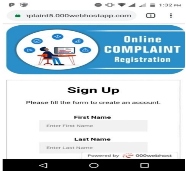
Fig.5. Registration Form.
