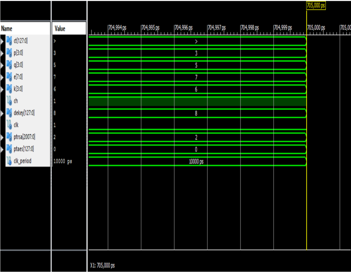
Fig 7: Simulation results of RSA algorithm
