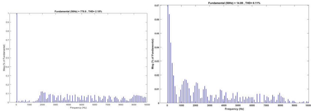
Fig.11 THD of output voltage and current with LS-PWM when modulation index is 1 and load is 50\Omega and 50mH
