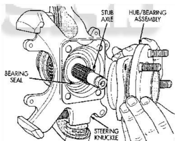
Fig. 2. Component of wheel hub and upright as reported by reference. [26]
