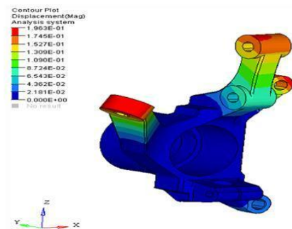
Fig. 9. Displacement Contour Of the Modified Model as per presented by ref. [20]
