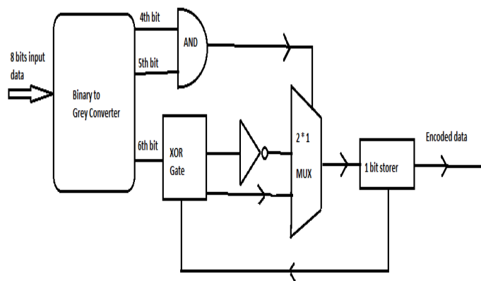
Fig. 3. Encoder of link design II.
