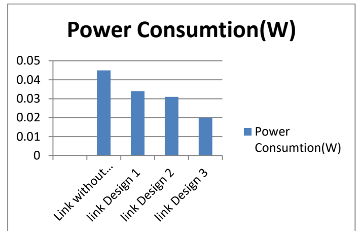
Fig.19 Comparison of power consumption of link designI,II,III.
