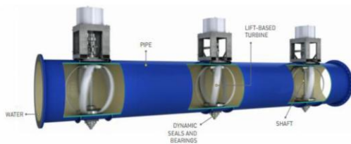
Figure1.1 System installed by Lucid company
