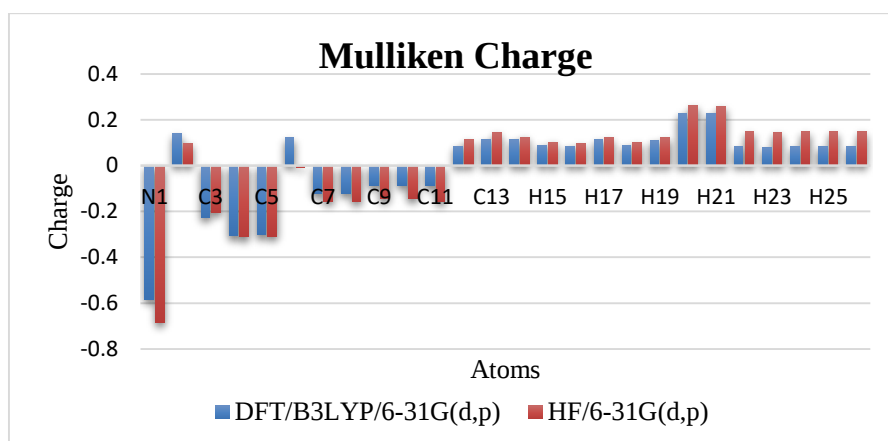
Fig.6. Muliken's atomic charges of 2-methyl-1phenylpropan-2-amine
