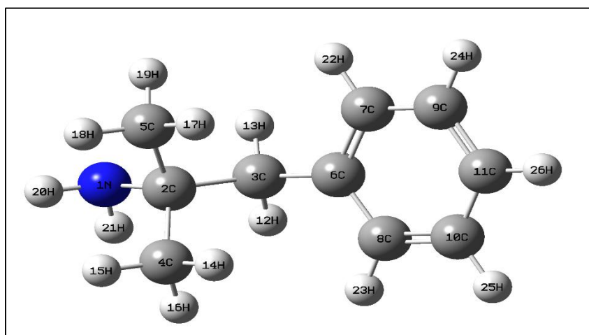
Fig.1 Optimized structure of 2-methyl-1-phenylpropan-2-amine
