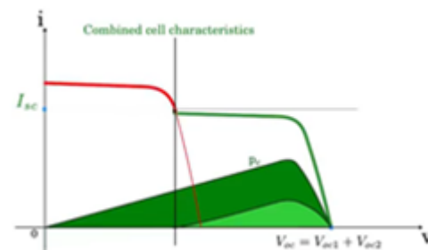
Fig.6. Improving solar efficiency by putting bypass diode
