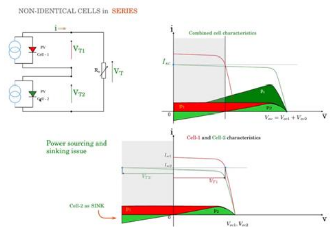
Fig.5.Solar PV cell in series along with Power characteristics
