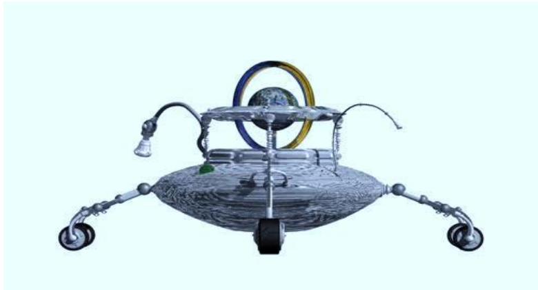
Fig.4:DentalNanorobots[49,50].
