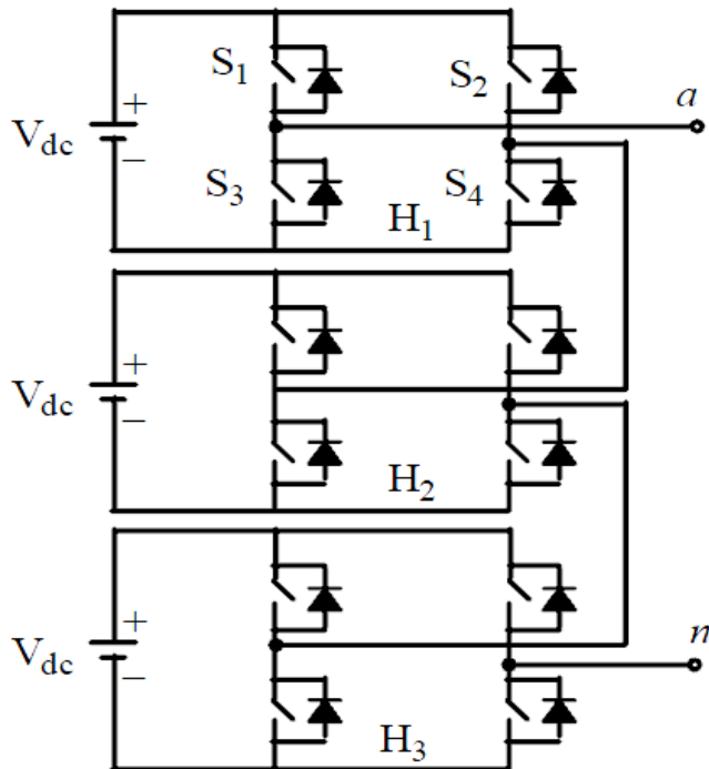
Fig-1: Configuration of Seven Level Cascaded Inverter
