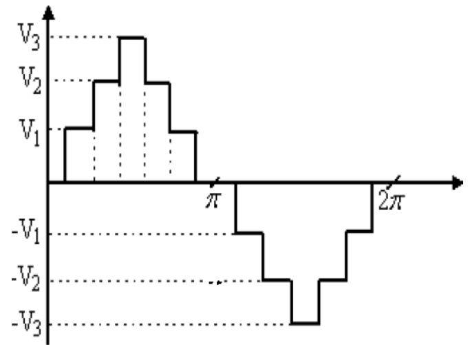
Fig-2: Typical Output Voltage Produced by Seven Level Cascaded Inverter
