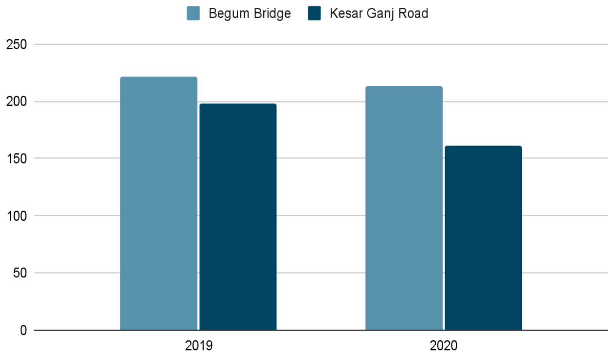
GRAPH (3.3) ANNUAL PM10 LEVELS OF MEERUT
