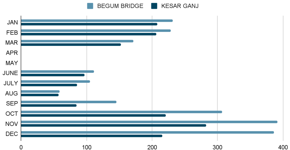
GRAPH (3.1) MONTH WISE RATE OF PM10 IN 2020
