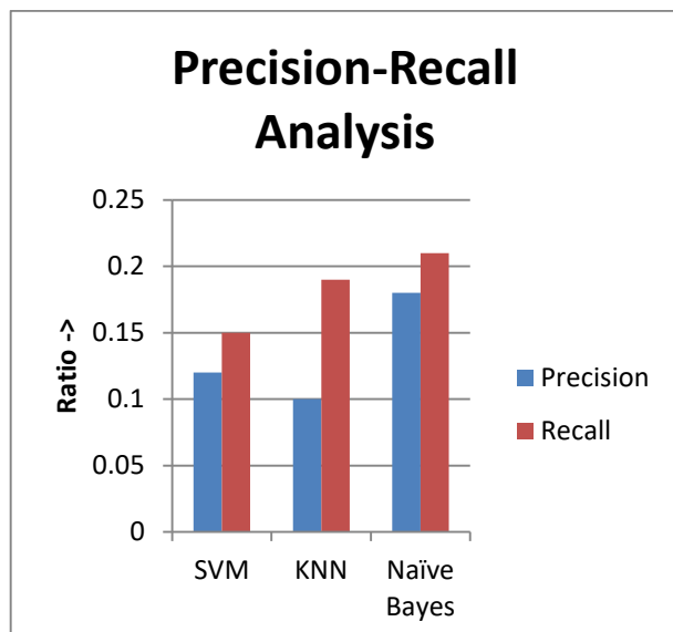
Figure 4: Precision-Recall Comparison
