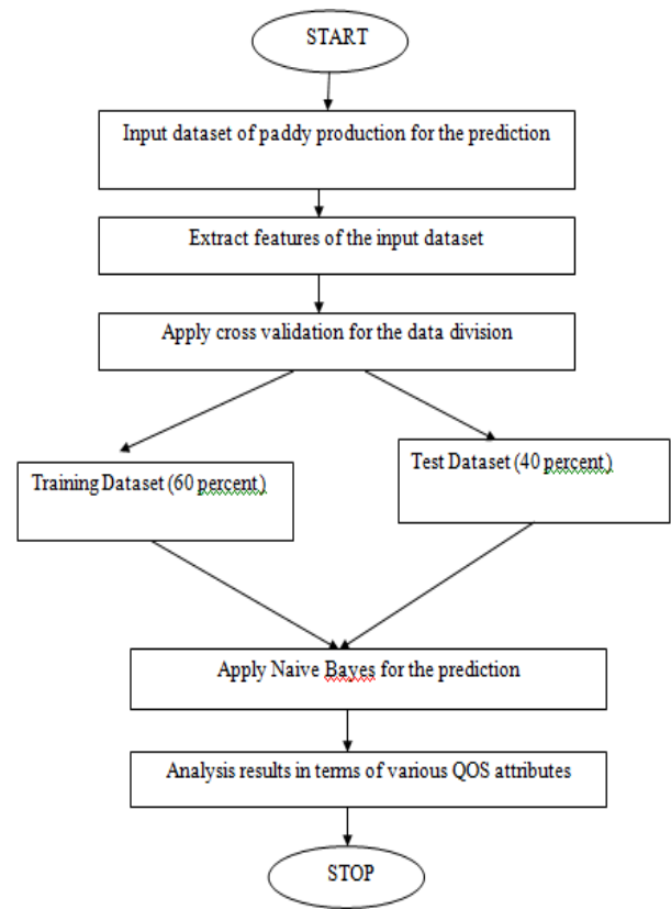
Figure 1: Proposed Flowchart
